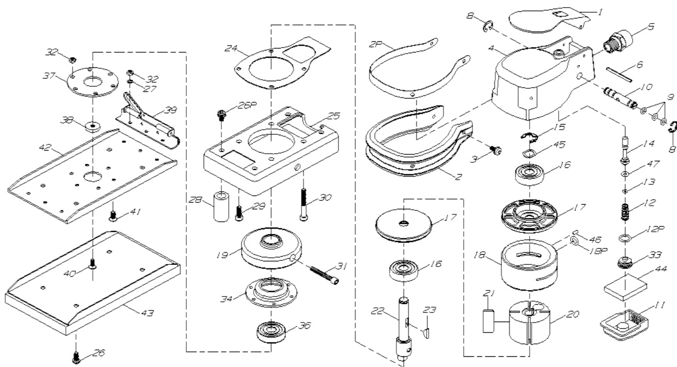
KI-6301 HEAVY DUTY AIR ORBITAL BLOCK SANDER
